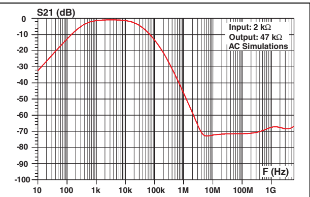
Figure 5. Attenuation simulation with 2 k \Omega input and 47 k \Omega output
