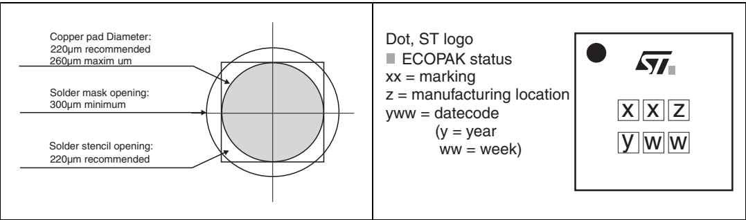
Figure 12. Footprint recommendations Figure 13. Marking
